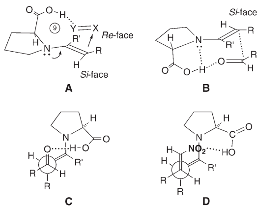
Re/Re -coupling of trigonal centers
