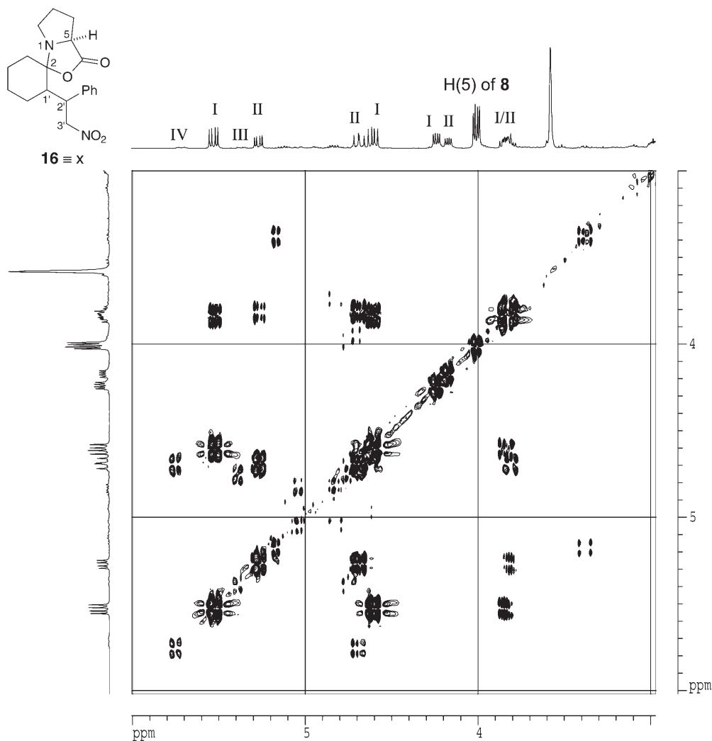
Fig. 3. Section from 3–6-ppm region of the 400-MHz 2D - ^1H -NMR spectrum of a reaction mixture of oxazolidinone 8 and \beta -nitrostyrene in (D_8)THF in an NMR tube. The four lowest-field dd signals I, II, III, IV arise from one of the \alpha - NO_2 - CH_2 H-atoms H(3'). Clearly, there are two major (I and II) and two very minor diastereoisomers (III and IV). The dd sets from the second \alpha - NO_2 - CH_2 H-atoms H(3') of the two major diastereoisomers appear at higher field (4.7 and 4.6 ppm). The benzylic H-atoms H(2') of the diastereoisomers are observed around 3.8 ppm. The characteristic dd signal of the bridgehead H-atom in the starting material 8 is detected at 4.0 ppm, and there are two additional dd signals at 4.25 and 4.18 ppm arising from H(5) of the product oxazolidinones, in a ratio matching that of the two sets from the \alpha - NO_2CH_2 H-atoms. From comparison of the intensities of these bridgehead-H-atom signals, it is suggested that the ratio of product 16 ( \equiv x ) and starting material 8 is close to 1:1 at the point in time of the measurement.
