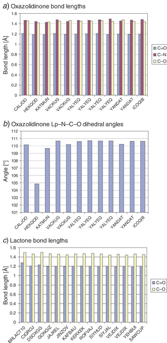
Fig. 6. Comparison of oxazolidinones and lactones with bicyclo[3.3.0]octane skeletons in crystal structures. a) C=O, C–N, and C–O bond lengths in oxazolidinones; b) virtual (lone-pair)–N–C–O dihedral angles in oxazolidinones (cf. Fig. 5, c, left-hand side); c) C=O and C–O bond lengths in bicyclic lactones are essentially identical to those in oxazolidinones (cf. a). Data from the Cambridge Crystallographic Database as of September 2006.
