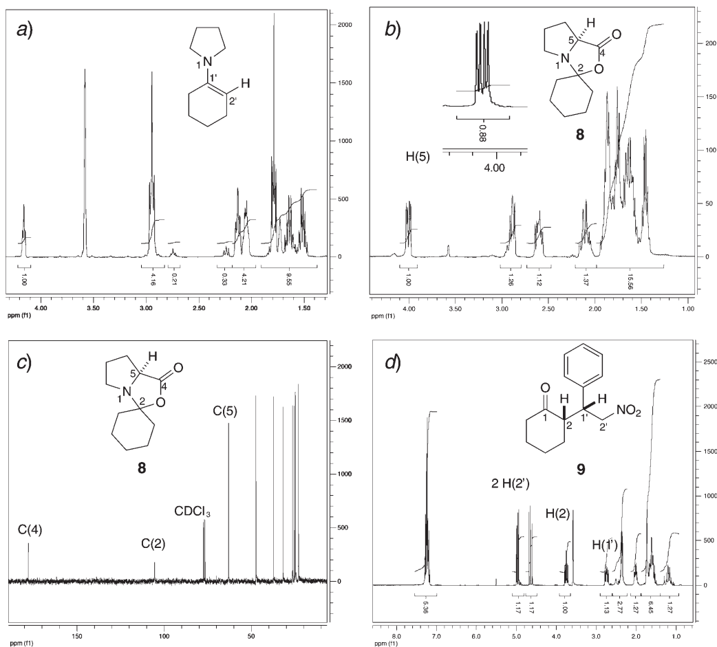
Fig. 1. NMR Spectra of oxazolidinone 8 ( ^1\text{H-NMR} in (\text{D}_8)\text{THF} , ^{13}\text{C-NMR} in \text{CDCl}_3 ; b and c), of 1-(cyclohex-1-enyl)pyrrolidine in (\text{D}_8)\text{THF} (a), and of nitro ketone 9 in (\text{D}_8)\text{THF} d). Compound 9 was isolated after reaction of 8 with \beta -nitrostyrene in THF and aqueous workup. Only the characteristic low-field signals are assigned in these presentations (cf. [29a][30a], the data of the 2D-NMR spectrum of Fig. 3, and the Exper. Part ). The ^1\text{H-NMR} spectra shown here were recorded in (\text{D}_8)\text{THF} , because the reaction of 8 with \beta -nitrostyrene was performed and NMR-spectroscopically followed in this solvent (Fig. 3). The small signal in b) at 4.15 ppm arises from a trace of the pyrrolidino-enamine (cf. a)) in the oxazolidinone 8 sample used.
