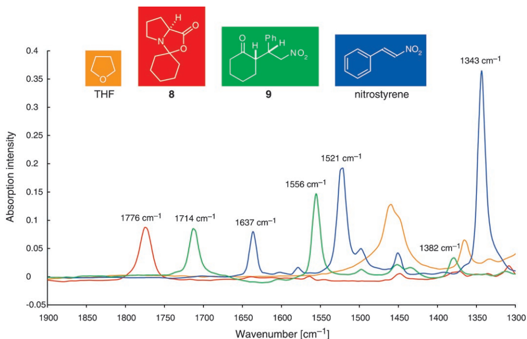
Fig. 2. Section from the 1900–1300- \text{cm}^{-1} region of the IR spectra of THF (orange), of the oxazolidinone 8 (red), of \beta -nitrostyrene (blue), and of the nitro ketone 9 (green). The spectra were recorded as THF solutions, and the THF bands near 1460 and 1360 \text{cm}^{-1} were electronically removed. The same wavenumber section was used to follow the reaction of 8 with \beta -nitrostyrene in THF (see Fig. 4).
