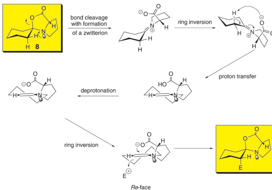
Scheme 12. Reaction of the Tricyclic Spiro-oxazolidinone 8 with an Electrophile in Analogy to the Process Outlined in Scheme 11 for an Unsymmetrical Ketone Derivative
