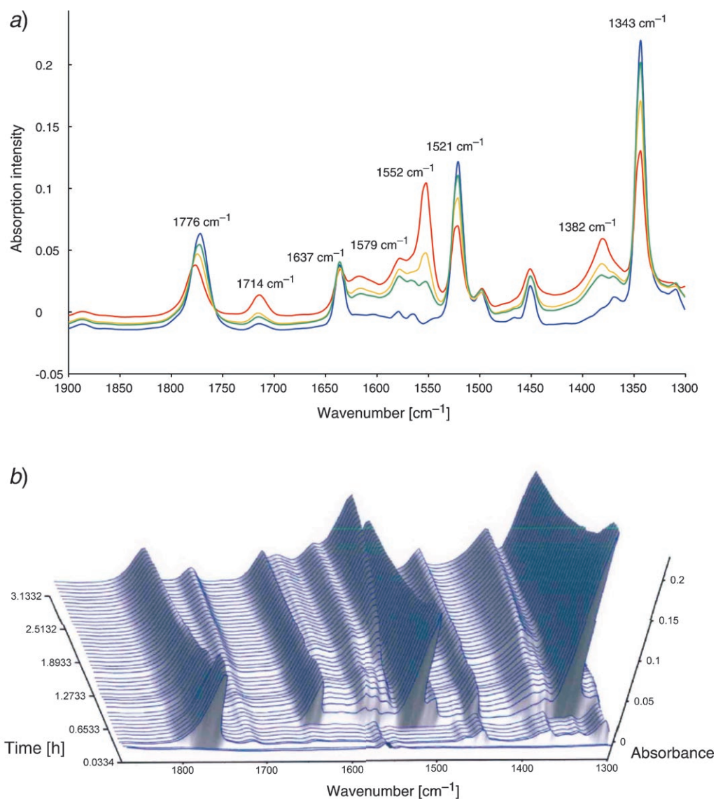
Fig. 4. Course of the reaction of oxazolidinone 8 with \beta -nitrostyrene (in (D 8 )THF from 0° to room temperature) followed by IR spectroscopy ('ReactIR'). Clearly, the characteristic oxazolidinone IR absorption near 1775 cm -1 does not disappear as the reaction proceeds. The band at 1714 cm -1 arising from nitro ketone 9 is an indication that moisture was not rigorously excluded from this experiment. For assignment of the various bands to the components of the reaction mixture, see also Fig. 2. a) Reaction times and temp.: 0 min, 0° (blue); 18 min, 10° (green); 48 min, 15° (orange); 150 min, room temperature (red); b) 3D presentation of the course of the reaction.
