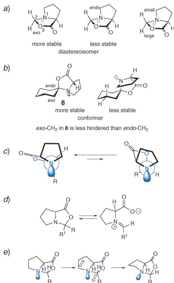
Fig. 5. Structures of oxazolidinones derived from proline. a) In aldehyde derivatives, the R group is preferentially in the exo -position, and the larger group of unsymmetrical ketones R–CO–R' resides on the exo -face of the bicyclo[3.3.0]octane skeleton; b) the exo -substituent of symmetrical ketones RCOR is less hindered than the endo -substituent, and in 8 the position of the O-atom is expected to be axial, and that of the N-atom equatorial; c) there is no lone-pair–(C–O) interaction in the most stable conformation of a bicyclic oxazolidinone; the conformation with such an interaction will be more strained. (cf. e); d) dissociative ring opening/closure of a bicyclic oxazolidinone; e) distortion of the more stable conformer to a more strained conformer with lone pair N → σ C–O * interaction.
